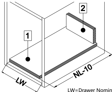
LW=Drawer Nominal Width NL=Nominal length
