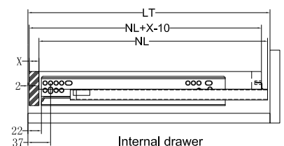
Internal drawer
