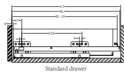
Standard drawer
