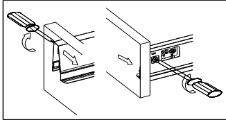
1 Installed panel Remember that tighten the fixing screw Front panel side adjustment right 1mm
