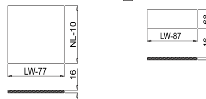
1 Drawer Bottom Dimensions (mm) 2 Drawer Back Dimensions (mm)
