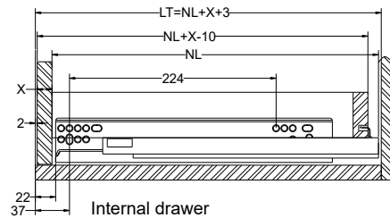
Internal drawer LT min=NL+X+3
