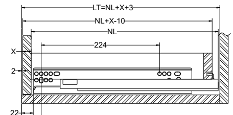
Internal drawer LT min=NL+X+3
