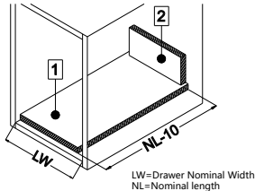
Technology pivot: Bottom and Back Panel Measurement 16MM Density Panel
