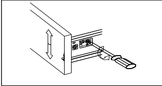
Front panel height adjustment \pm 2\text{mm}
