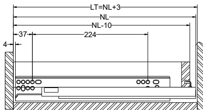
Standard drawer LT min=NL+3
