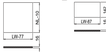
1 Drawer Bottom Dimensions (mm) 2 Drawer Back Dimensions (mm)
