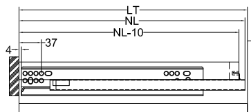
Standard drawer
